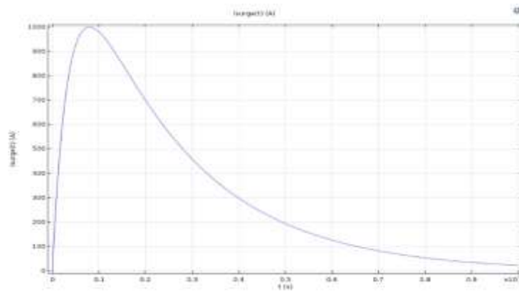
Figure 1 Typical 8/20 \mu s surge waveform
