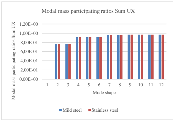
Figure 17. Graph G+2 building modal mass participating ratios sum UX
