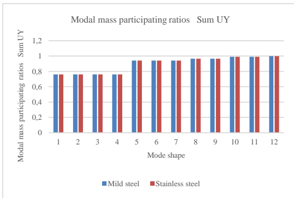
Figure 18. Graph G+2 building modal mass participating ratios sum UY
