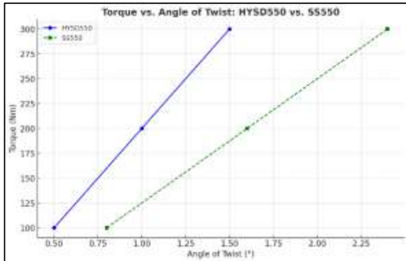
Figure 23. The above graph illustrates the torque vs angle of twist for both HYSD550 and SS550.
