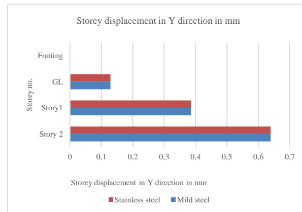
Figure 10. Graph G+2 building storey displacement in Y direction
