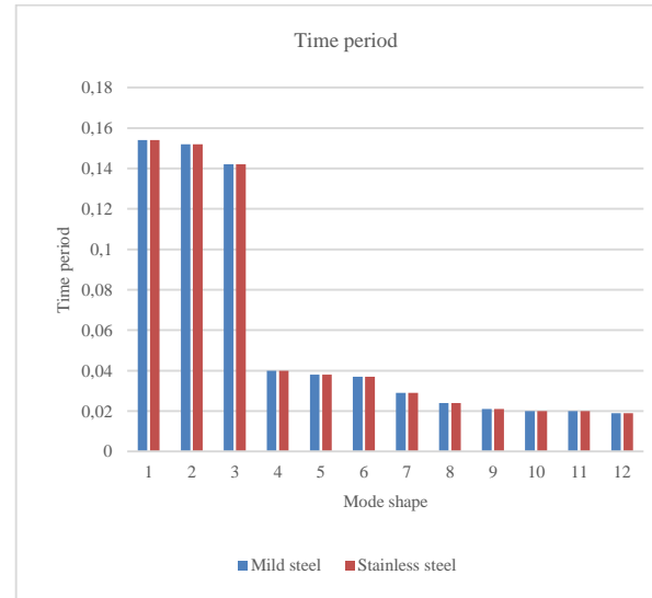
Figure 15. Graph G+2 building time period
