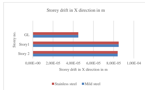
Figure 11. Graph G+2 building storey drift in X direction
