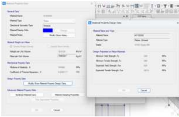
Figure 7. Input values of HYSD550 Reinforcements
