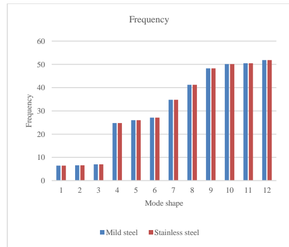
Figure 16. Graph G+2 building frequency
