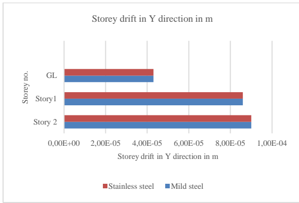
Figure 12. Graph G+2 building storey drift in Y direction
