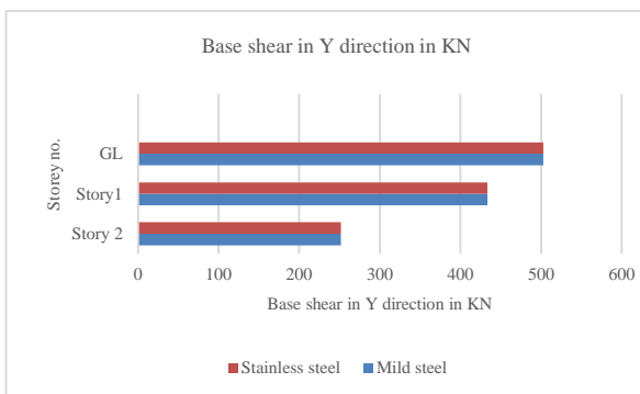
Figure 14. Graph G+2 building base shear in Y direction
