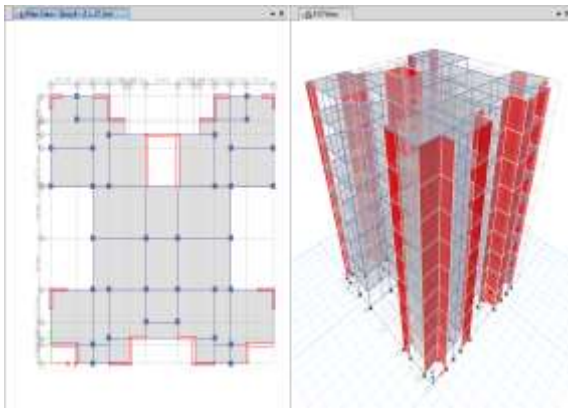
Figure 8. Plan & 3D view of the building
