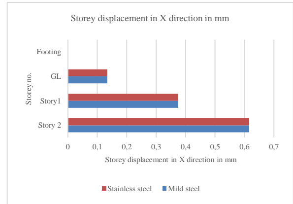
Figure 9. Graph G+2 building storey displacement in X direction
