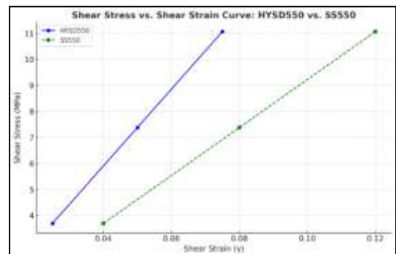
Figure 22. The shear stress versus shear strain plot shows the torsional behaviour between HYSD550 and SS550.
