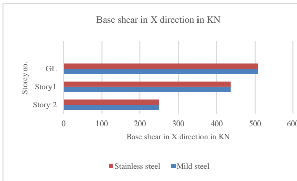
Figure 13. Graph G+2 building base shear in X direction
