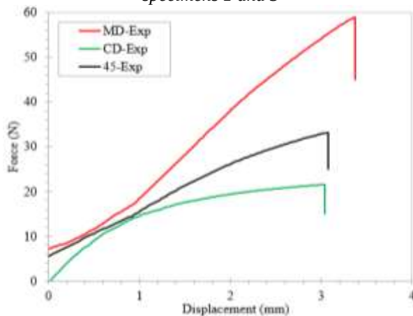
Figure 4. Force vs displacement relationship of paper specimen 2
