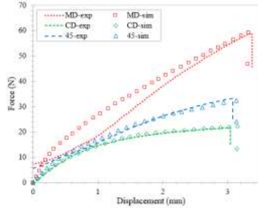
Figure 6. Experimental and numerical results of tensile test for specimen
