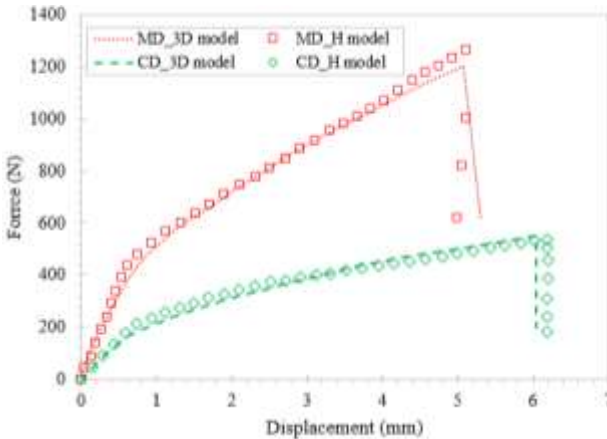
Figure 8. Comparison of the behavior of homogeneous and 3D panel
