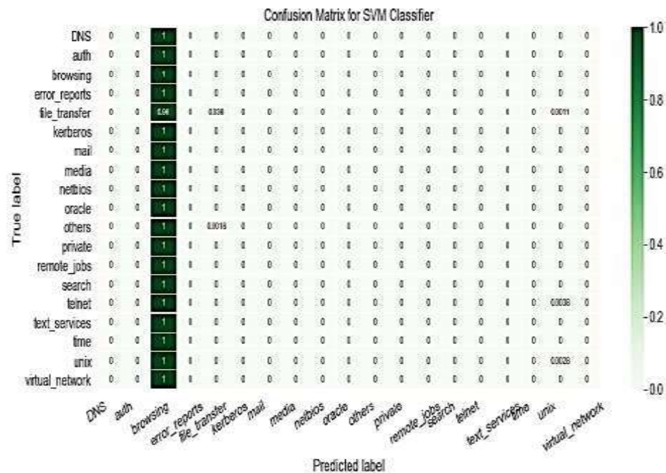
Figure 10. Confusion Matrix for SVM Classifier
