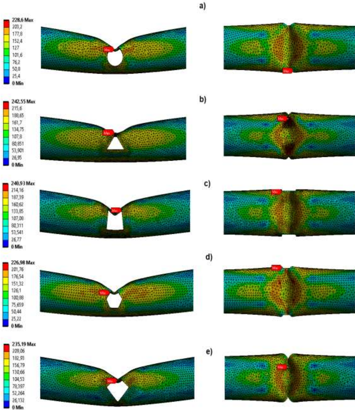
Figure 6. Von-Mises stress distributions of the tube with various hole shapes, a) circle, b) triangle, c) square, d) hexagon, e) diamond
