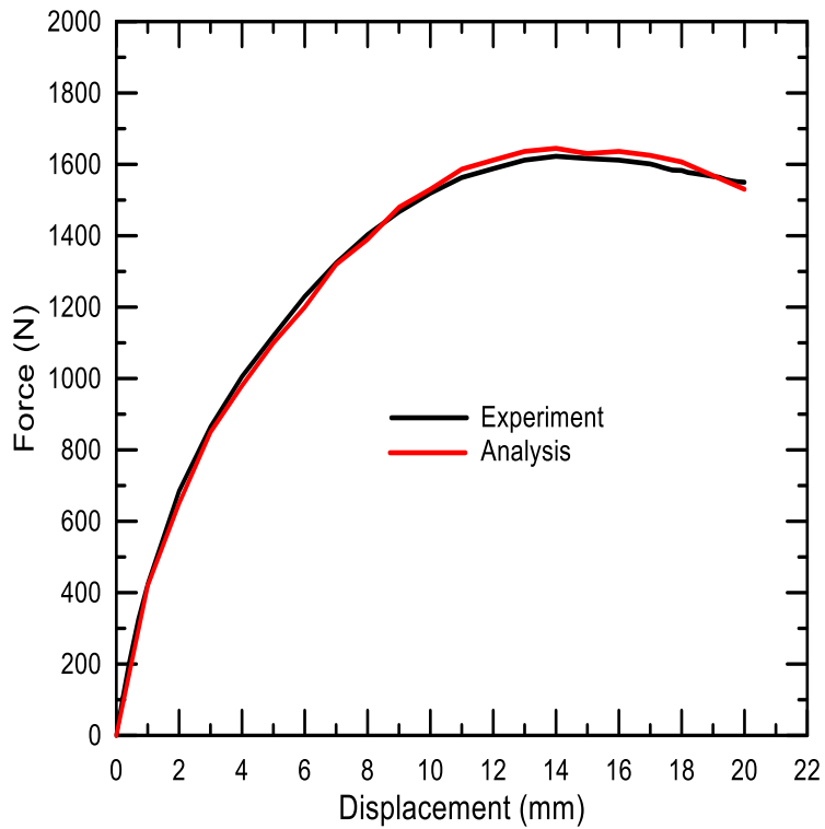
Figure 2. Force-displacement curves from the experiment and finite element simulation
