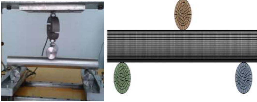
Figure 1. a) Experimental set-up for three-point bending validation test, b) Finite element analysis model
