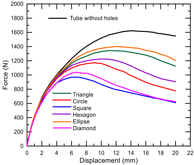
Figure 5. Force-displacement curves of tubes with various hole shapes
